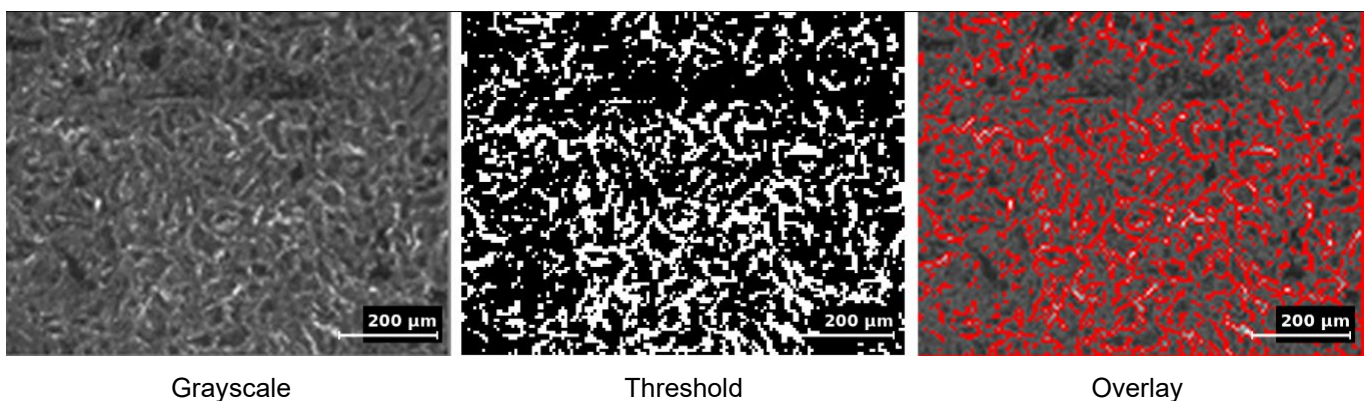
Fig. 8. Optical micrograph and ImageJ segmentation of the weld metal for the E6013–E6013 electrode combination at 50× magnification; scale bar = 200 μm
