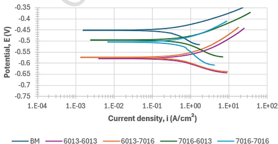
Fig. 18. Potentiodynamic polarization curves of the BM and SMAW-welded specimens measured on the capping surface in 3.5 wt.% NaCl solution
