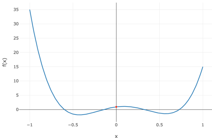
Fig. 2 – The example of a graphical representation of a special function.
