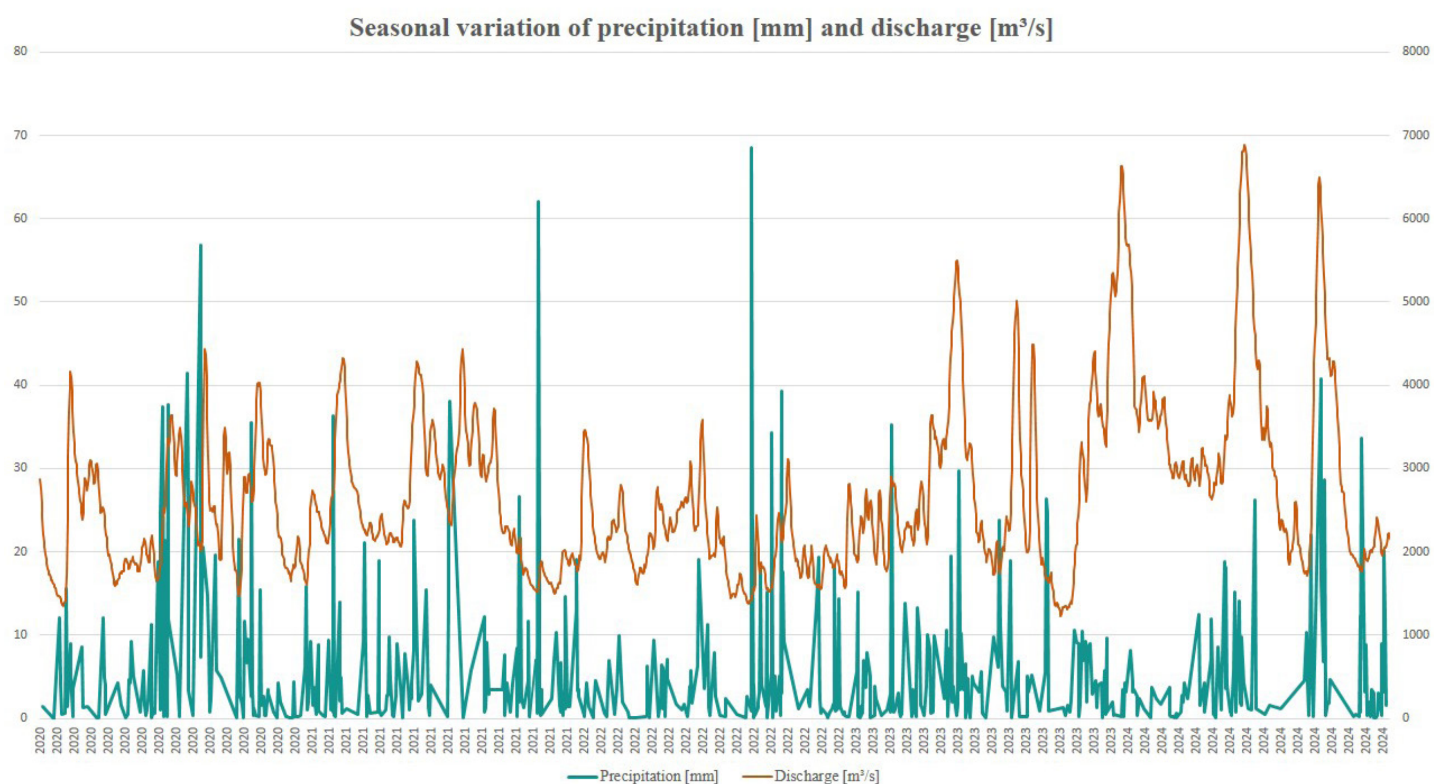
Figure 9. Seasonal variation of precipitation [mm] and discharge [m³/s] for period of 2020 to 2024
