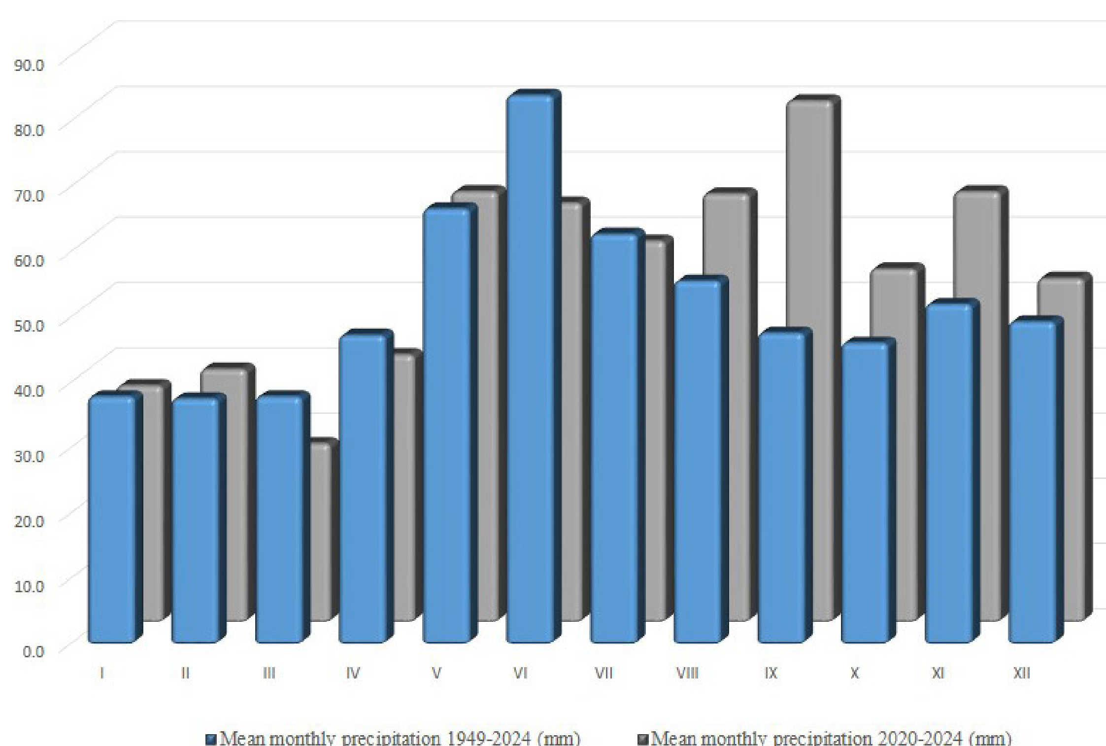
Figure 2. Comparison of mean monthly precipitation for the periods a) 1949–2024 (blue colour) and b) 2020–2024 (grey colour)
