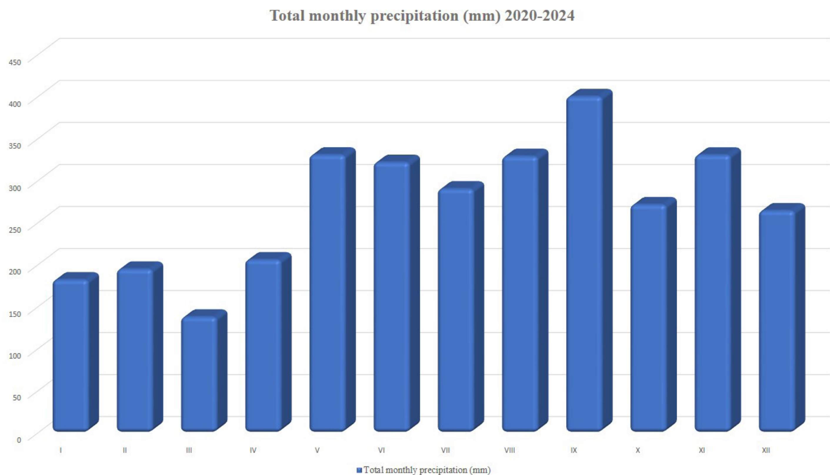
Figure 4. Trend of total monthly precipitation at the Rimski Šančevi station (2020–2024).
