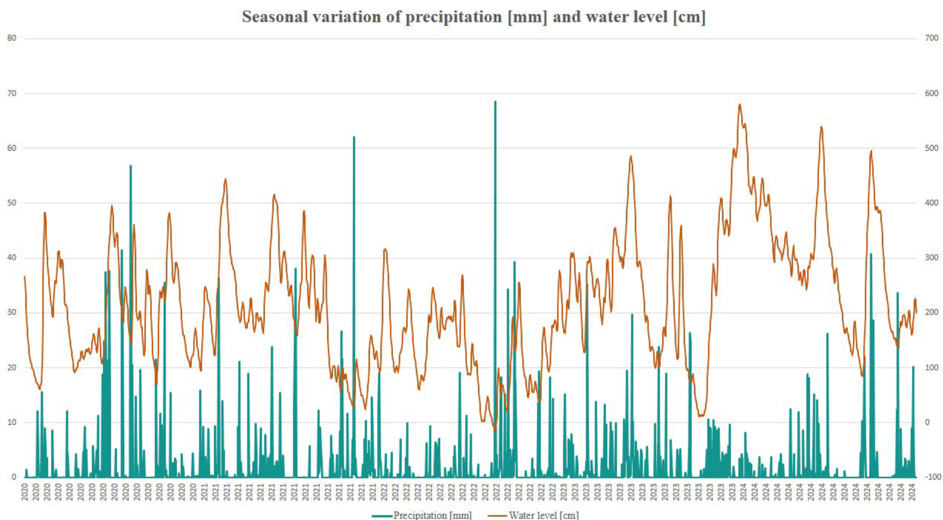
Figure 8. Seasonal variation of precipitation [mm] and water level [cm] for period of 2020 to 2024
