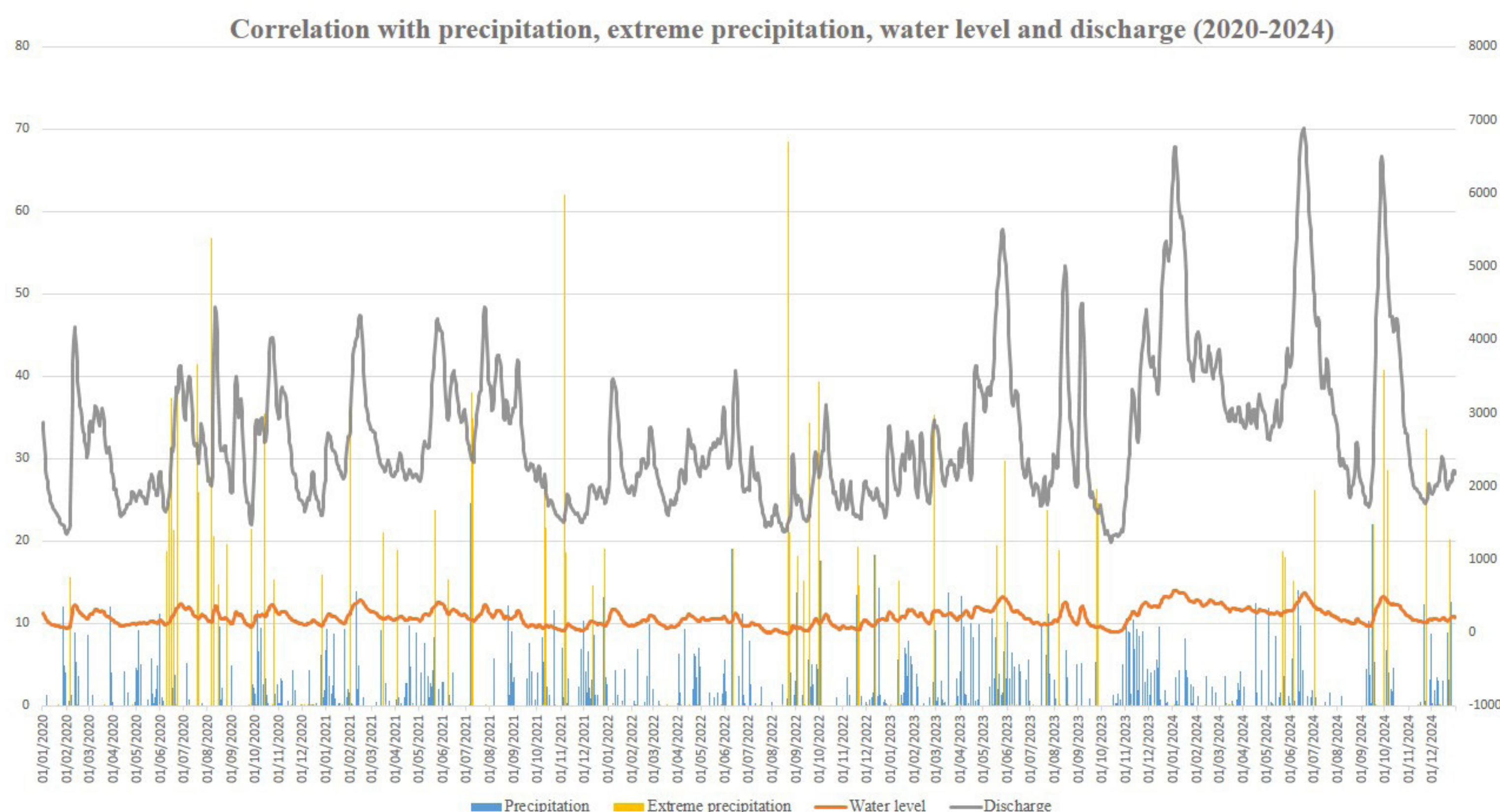
Figure 11. Correlation with precipitation, extreme precipitation, water level and discharge for 2020 to 2024.
