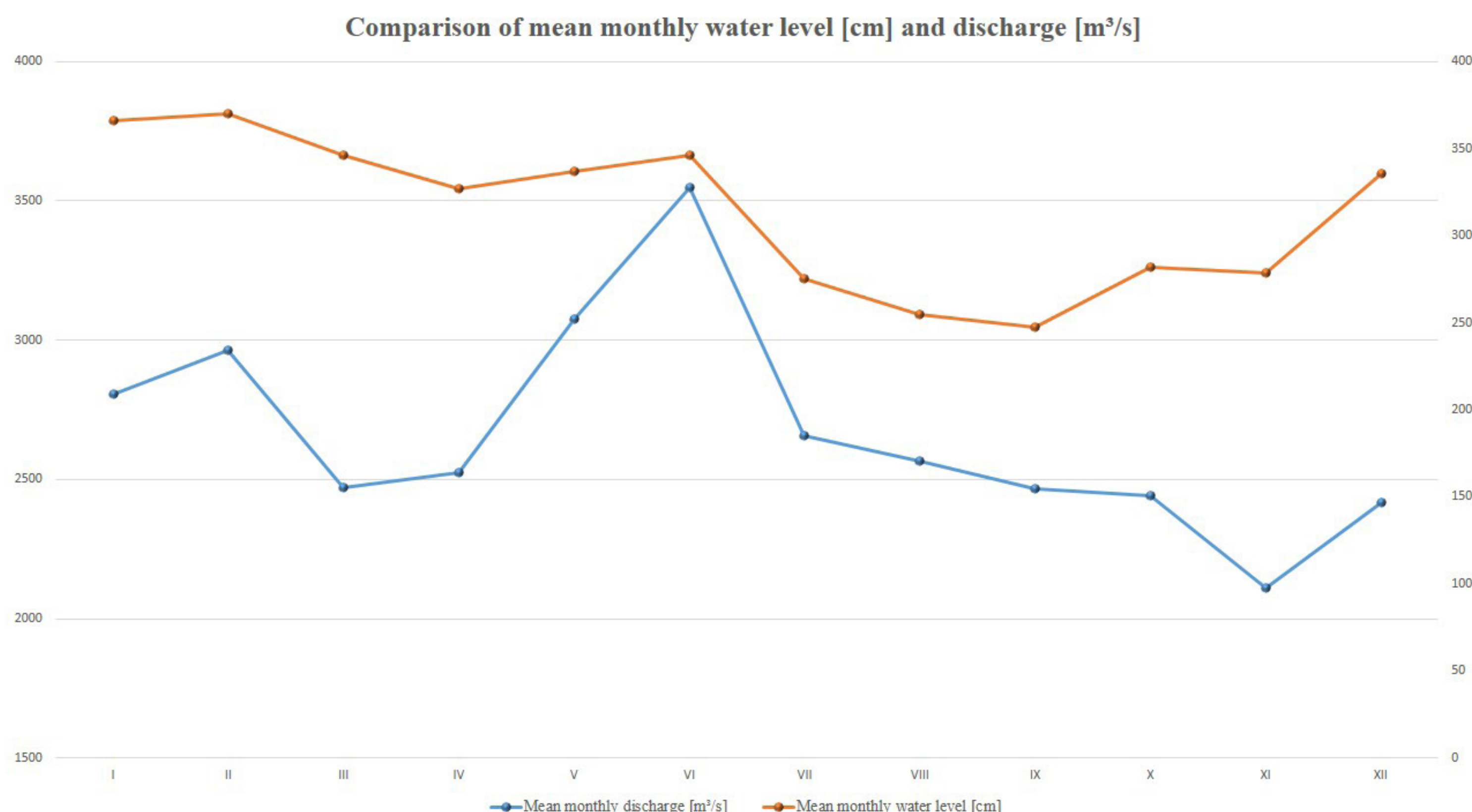
Figure 7. Comparison of mean monthly water level [cm] and discharge [ \text{m}^3/\text{s} ]
