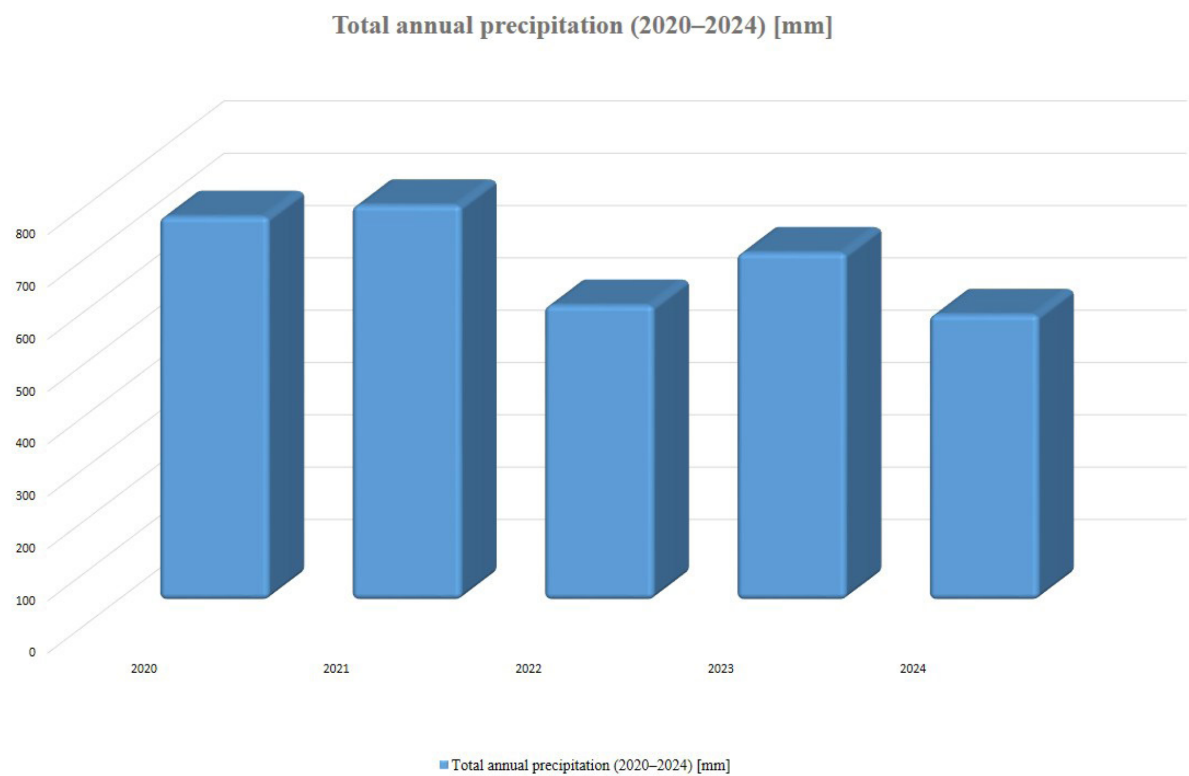
Figure 3. Trend of total annual precipitation at the Rimski Šančevi station (2020–2024).
