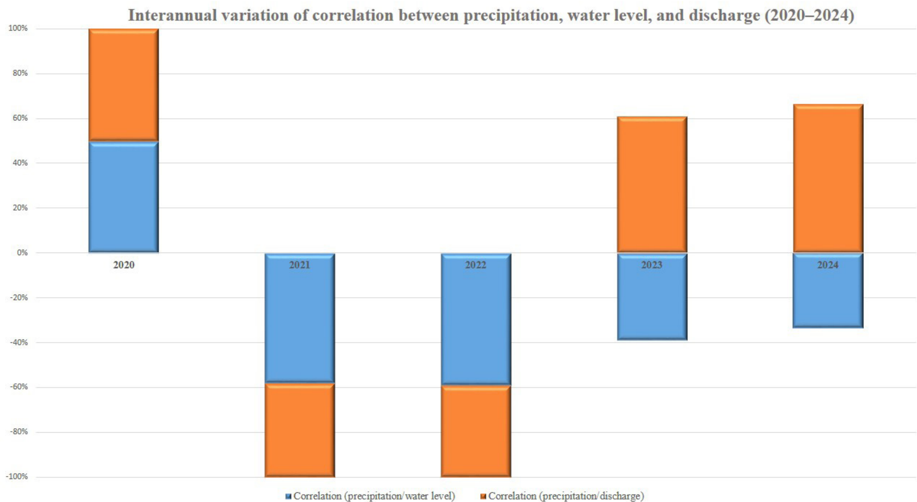
Figure 10. Interannual variation of correlation between precipitation, water level, and discharge (2020–2024) Source: RHSS, , Hydrological Yearbooks (2020-2024)
