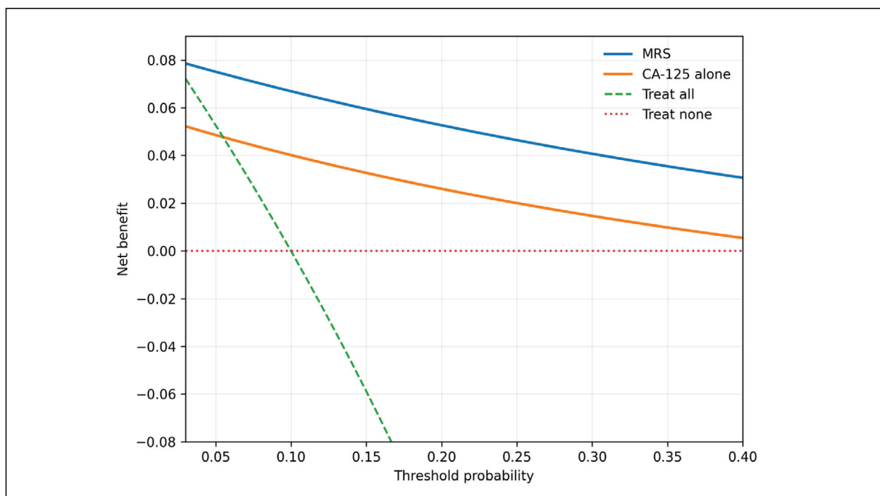
Supplementary Figure S2 Decision curve analysis of the multi-analyte risk score.
