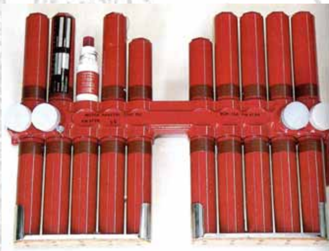
Figure 40. Pilot seat rocket motor for ORAO and G-4 aircraft
