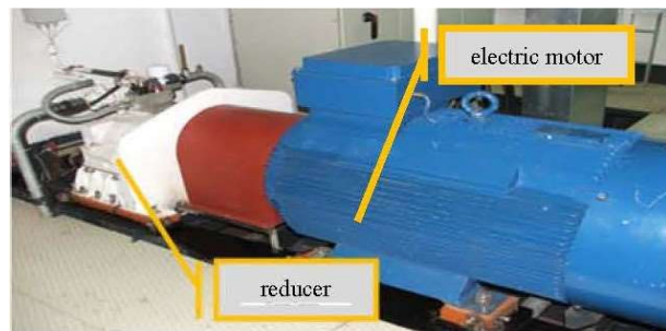
Figure 2. Selected electric motor behind the reducer
