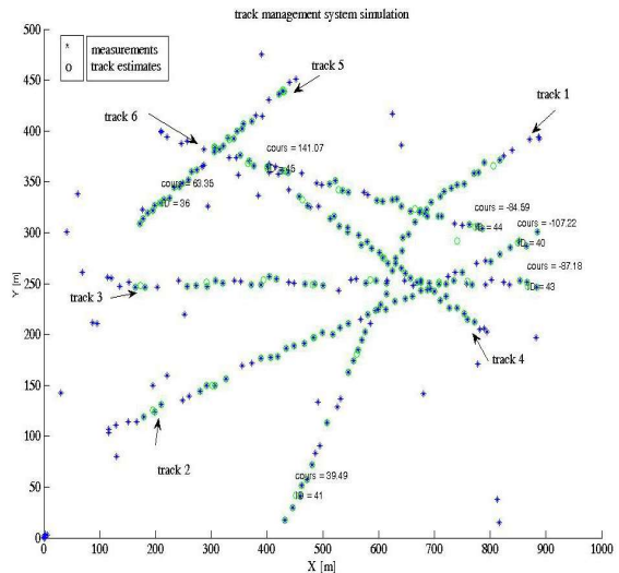
Figure 5. Simulations scenario of six targets
