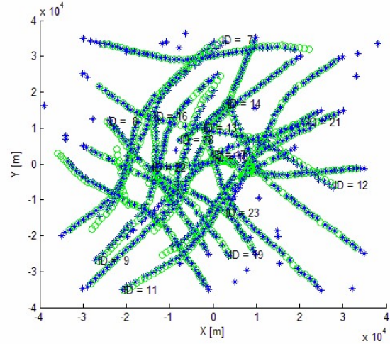
Figure 8. Simulations scenario of twenty targets
