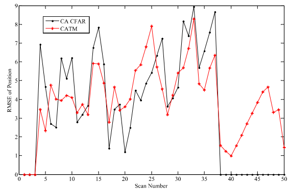
Figure 10. Comparative diagram RMSE of the position for overall (twenty) tracks (CATM CFAR versus CA CFAR)
