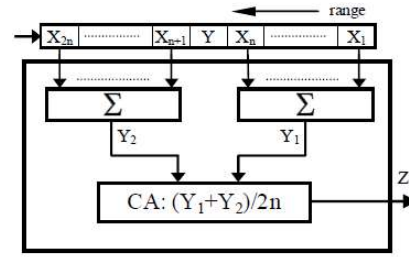
Figure 1. Block diagram CA-CFAR detector
