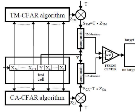
Figure 2. Block diagram of CATM-CFAR detector
