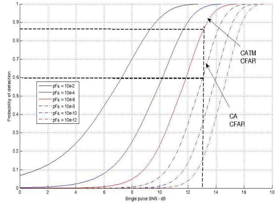
Figure 4. Parametric diagrams probability of detections versus signal to noise ratio (parameter probability of the false alarm)
