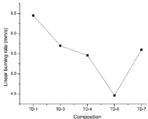
Figure 6. Average linear burning rate for selected pyrotechnic composition
