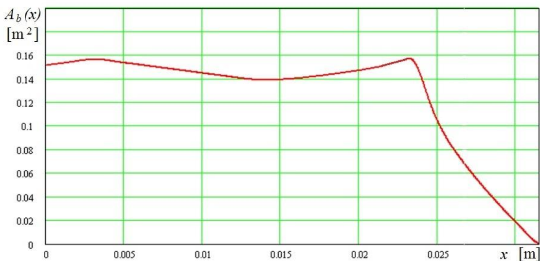
Figure 5. Burning area dependence from burned web, numerically calculated by SVOD software.
