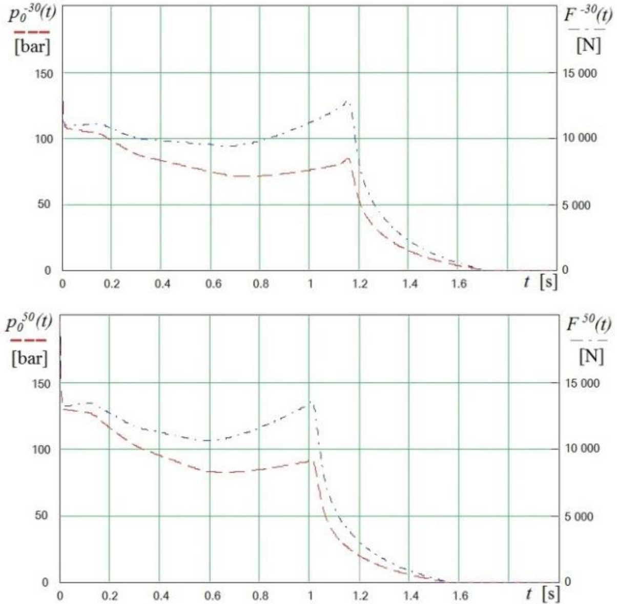
Figure 7. Calculated chamber pressure and thrust curves during the working time, on extreme ambient temperatures -30°C (above) and 50°C (below)
