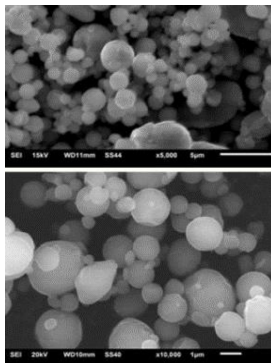
Figure 7. SEM images of nano-sized Al particles
