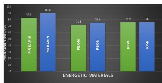
Figure 9. A graphic illustration of combustion efficiency for selected EM samples with micro and nano Al
