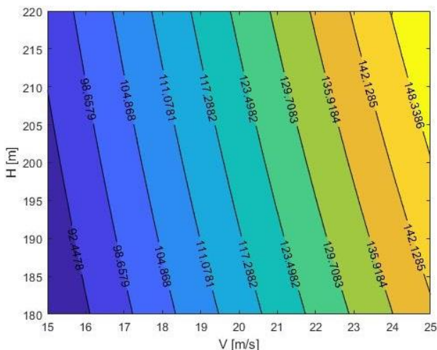
Figure 5. Flight path distance with changing airspeed and altitude
