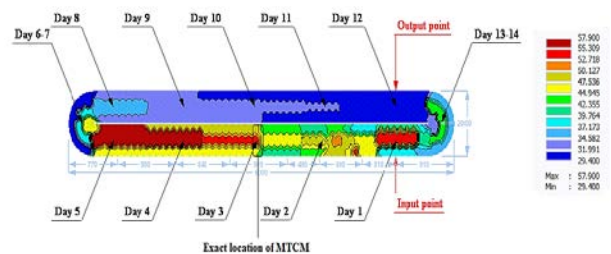
Figure 5. The temperature distribution model of the fermentation system (June 2019)
