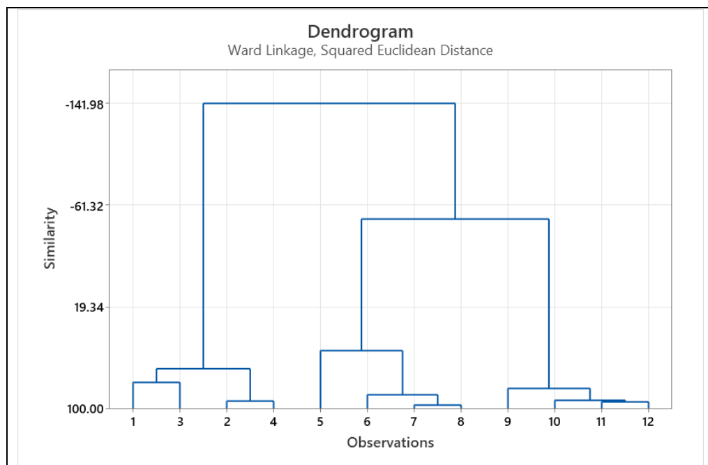
Figure 2. Dendrogram of Element Binding
