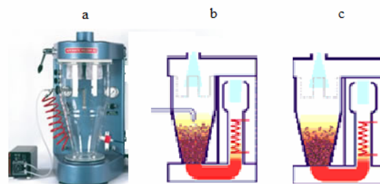
Fig. 1. STREA 1™ fluidized bed agglomerator/spray drier/coater ( http://www.niroinc.com )
