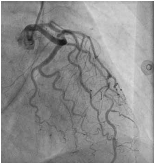
Fig. 1 LAD dissection
