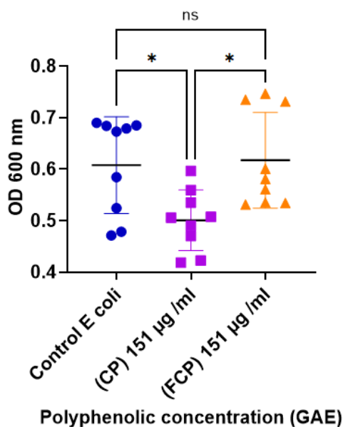
Figure 6. Comparison between similar polyphenolic concentrations extracted from AP and FAP against E.coli F4 (K88). Serial dilutions of CP and FCP extracts with varying total polyphenol (TP) concentrations were prepared, and the bacterial growth inhibition was monitored over 27.5 hours. The inhibition was tracked by measuring the optical density at 600 nm at 30-minute intervals
