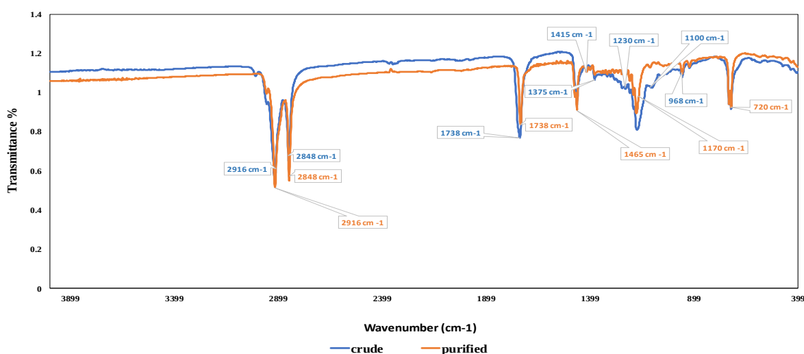
Figure 4. FTIR spectra of sunflower wax before and after purification
