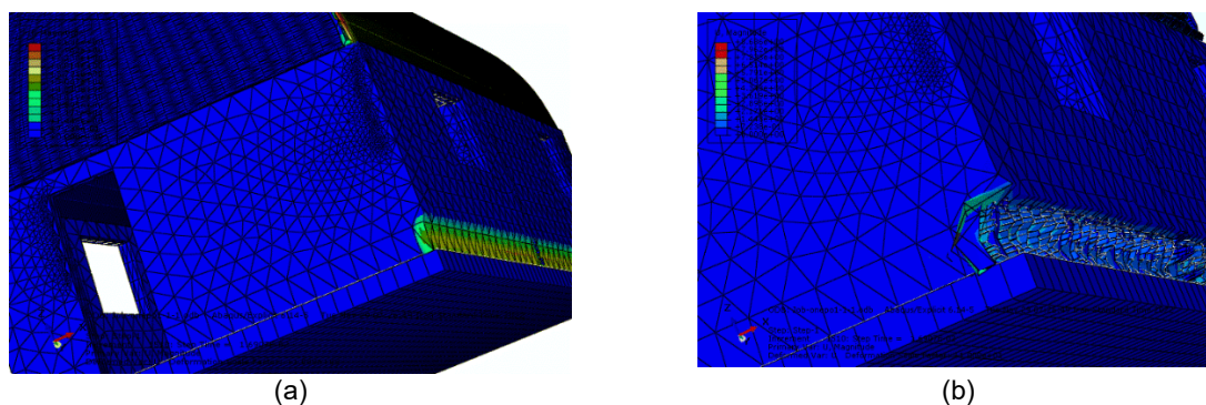
Figure 15. Shear damage to the foot of the walls under earthquake loading in the longitudinal direction of the structure: a) damage contours; b) magnified image of the wall's damage
