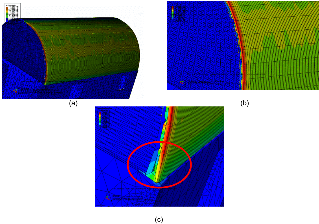
Figure 14. Seismic excitation on the length of the building, a. damage to the arch, b. damage to the grids between the windows, c. slipping of the arch over the living room
