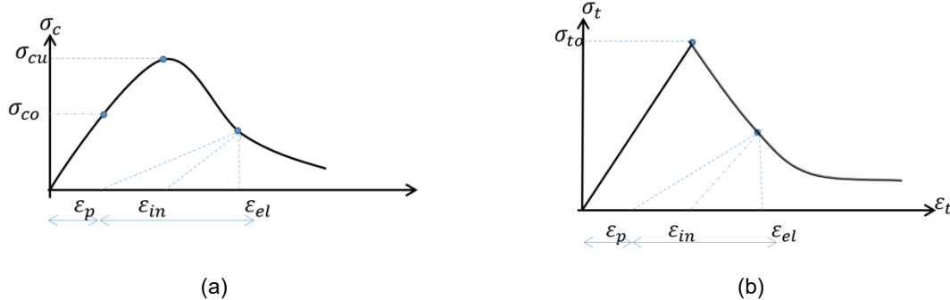
Figure 2. Concrete behavior: a) incompression; b) intension [45]
