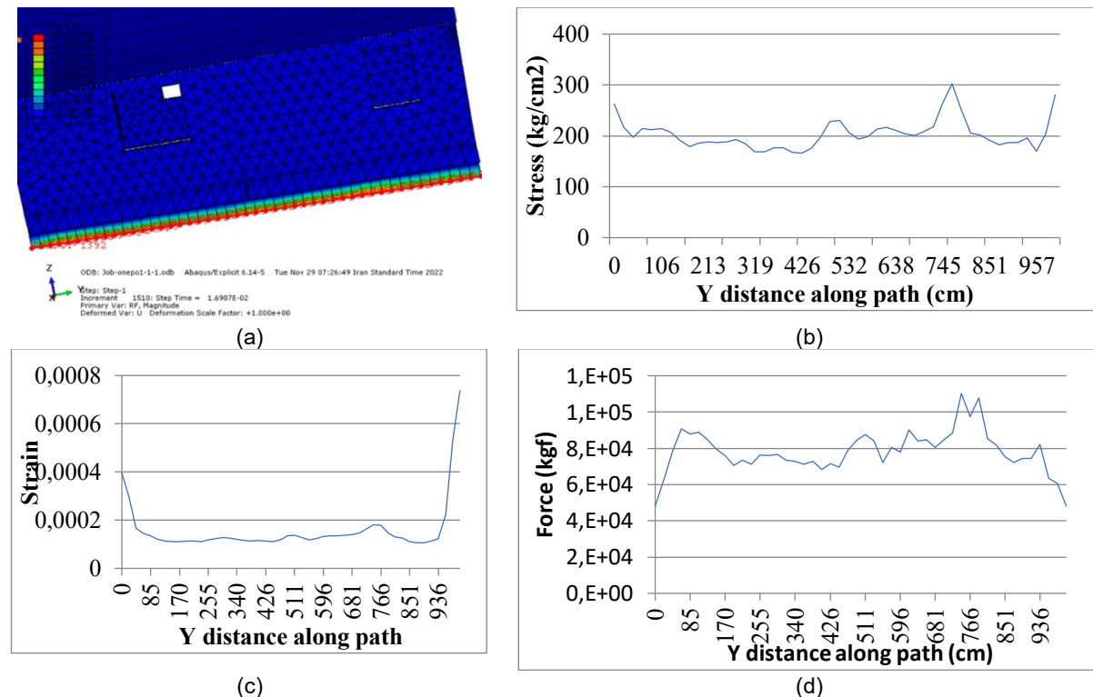
Figure 12. a) The considered path on the support; b) stress in the y direction; c) plastic strain, d) support reactions
