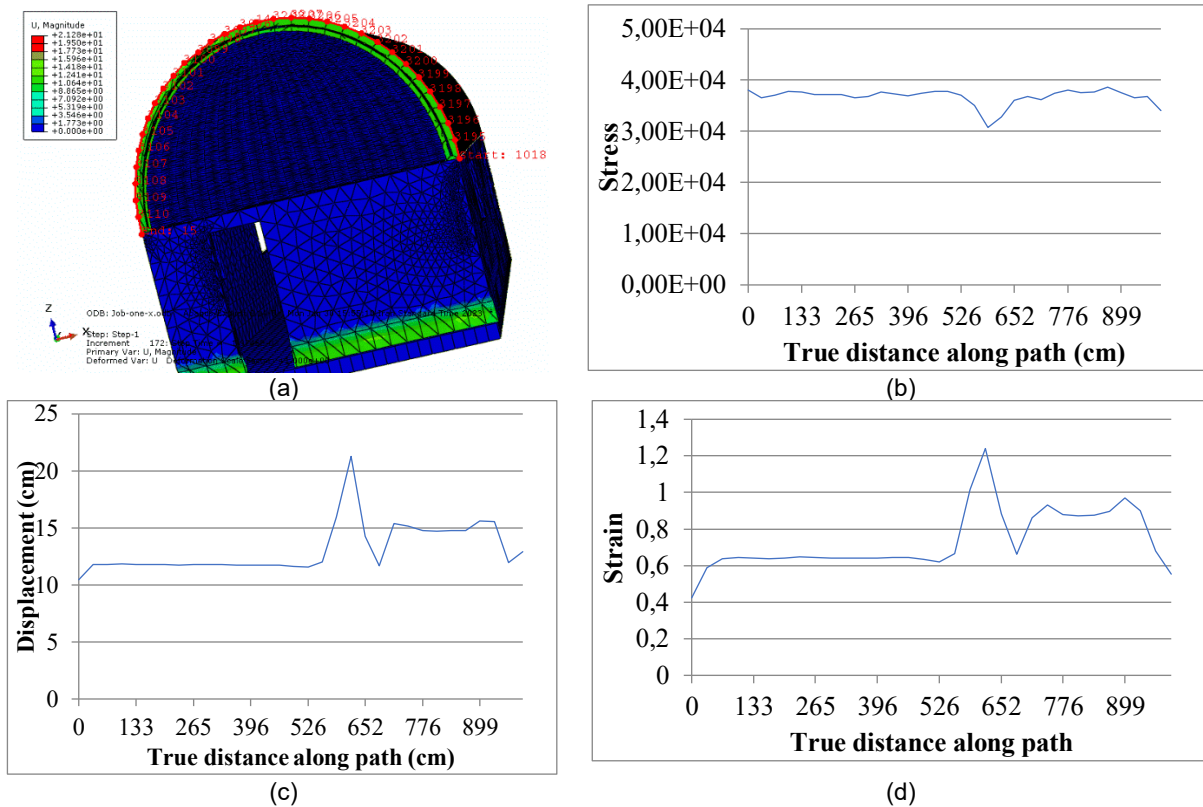
Figure 13. a) The considered path on the arch; b) von Mises stress; c) displacement; d) strain in the radial direction
