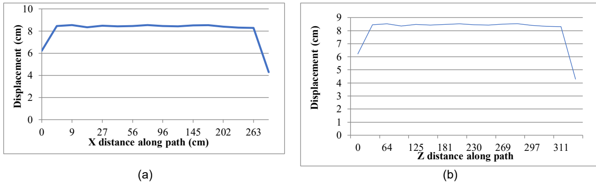
Figure 9. Displacement variations in the arch proportional to the distance from the beginning of the arch in the: a) x-direction; b) z-direction
