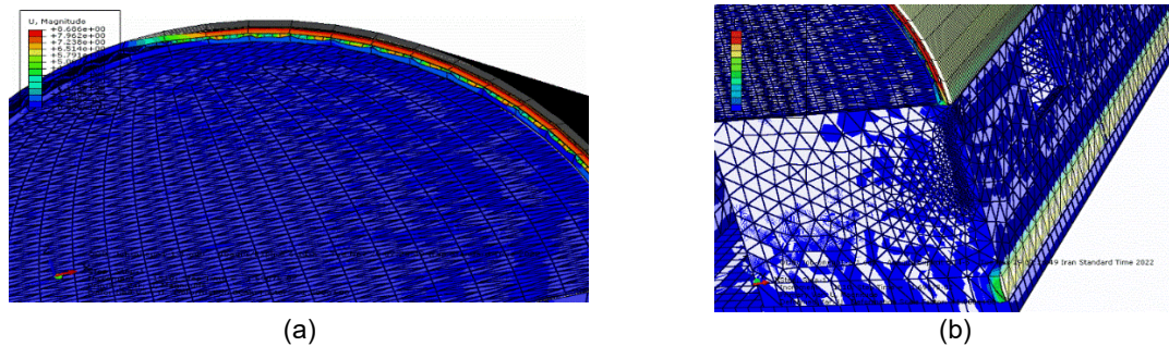
Figure 7. Deformed and undeformed elements of: a) the arch; b) the body of the structure
