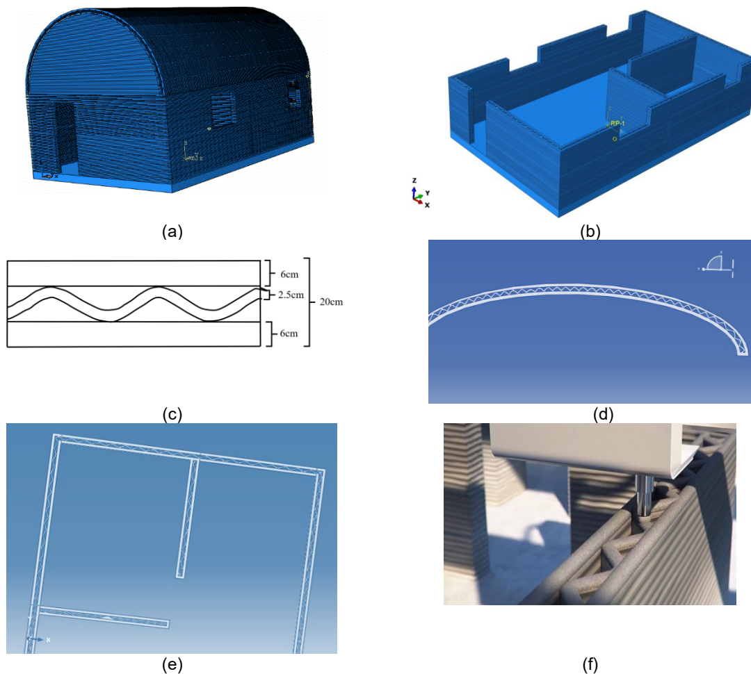
Figure 1. Finite element model of the considered building in this study: a) 3D-printed building; b) building plan; c) cross-section of the arch and walls; d) a layer of the modeled arch roof; e) a layer of the modeled walls; f) schematic printing process of the parallel filament with internal grids
