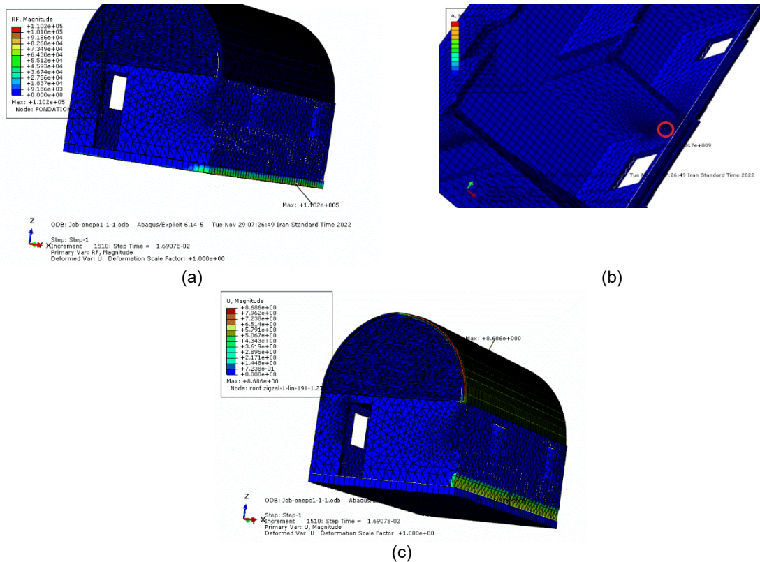
Figure 10. Extreme values of: a) support reactions; b) plastic strains; c) displacements
