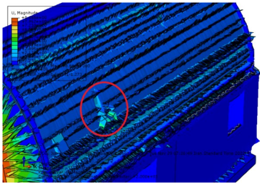
Figure 11. Maximum damage to the structure (magnified deformations)
