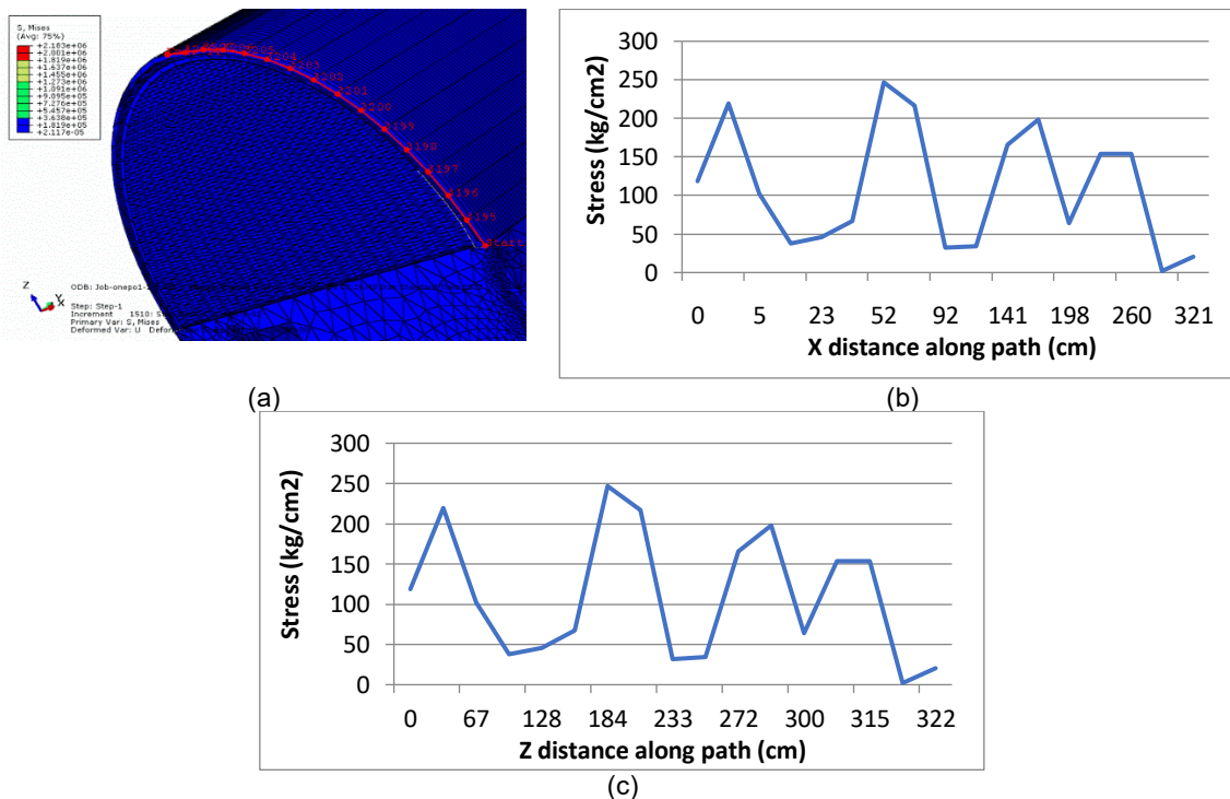
Figure 8. a) The considered path on the arch; b) von Mises stress variations in the x-direction; c) von Mises stress variations in the z-direction
