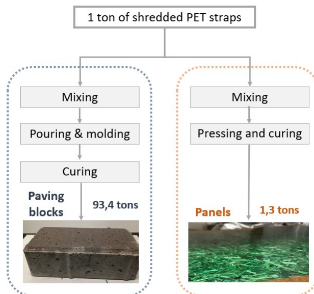
Figure 3. System boundaries for paving blocks and panels with shredded PET straps
