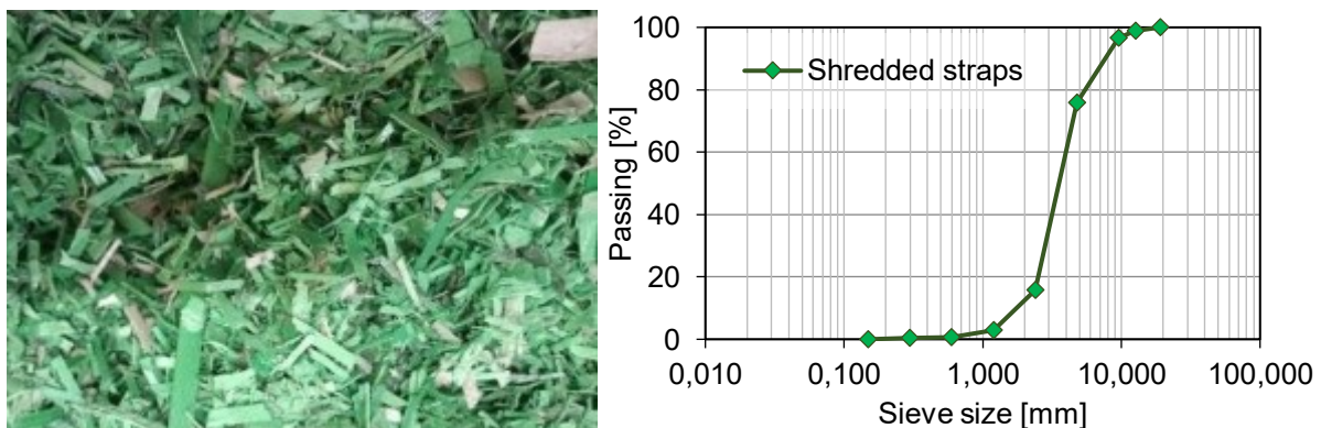
Figure 2. Shredded PET straps (left) and granulometric analysis of shredded PET straps (right)
