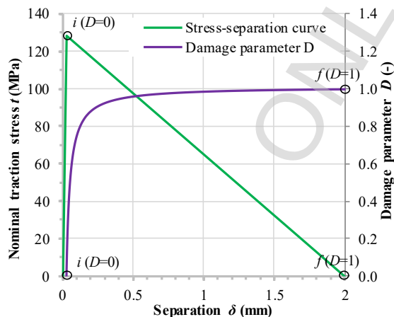
Figure 6. Cohesive contact for modelling rebar-to-coupler connection
