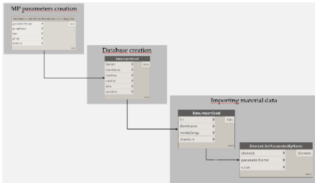
Figure 2. Dynamo workflow [19]
