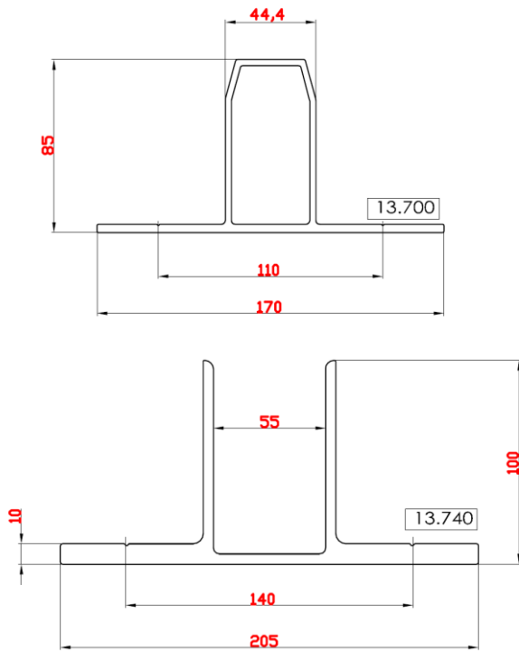
Figure 5. European Façade Product (EFP) 50 Façade System shoe brackets catalogue drawings (top) 13700 with size 170 × 85 and (bottom) 13740 with size 205 × 100
