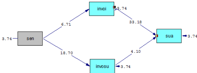
Fig. 1. path analysis and path coefficients of the model resulted from LISERL software based on subsidiary variables
