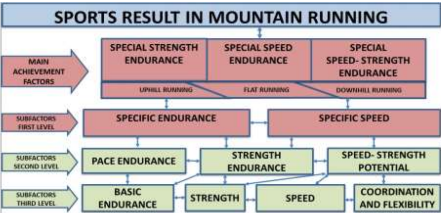
Figure 1. Model of the sports result in mountain running.
