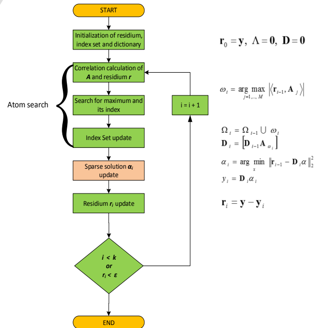
Figure 4. Algorithm for orthogonal matching pursuit.
