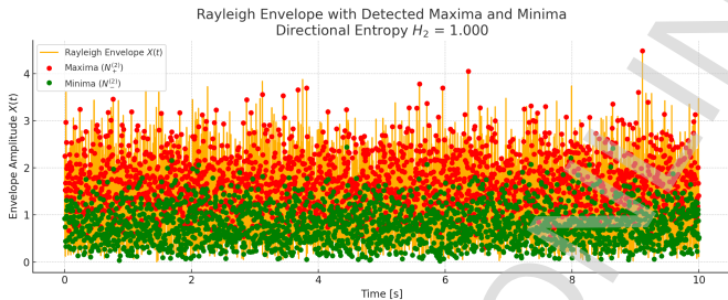
Figure 3. Rayleigh fading envelope with identified local extrema over time.
