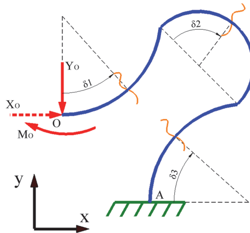
Figure 5: Displacement point O in the horizontal and vertical direction within a quarter of the m2D-AS
