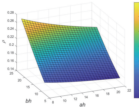
Figure 6: Effects of the parameter ah and bh on relative density \rho_r
