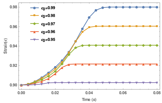
Figure 8: Effects of varying initial strain \varepsilon_0 on material response \varepsilon_0 = 1, \alpha = 10, \omega_0 = 2, \lambda = 2
