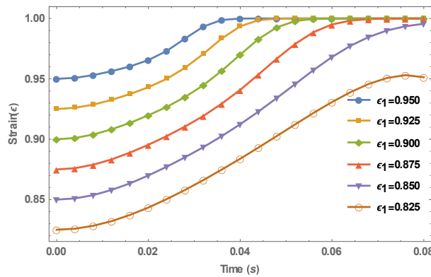
Figure 9: Effects of varying strain on material response \varepsilon_0 = 1, \alpha = 10, \omega_0 = 2, \lambda = 2
