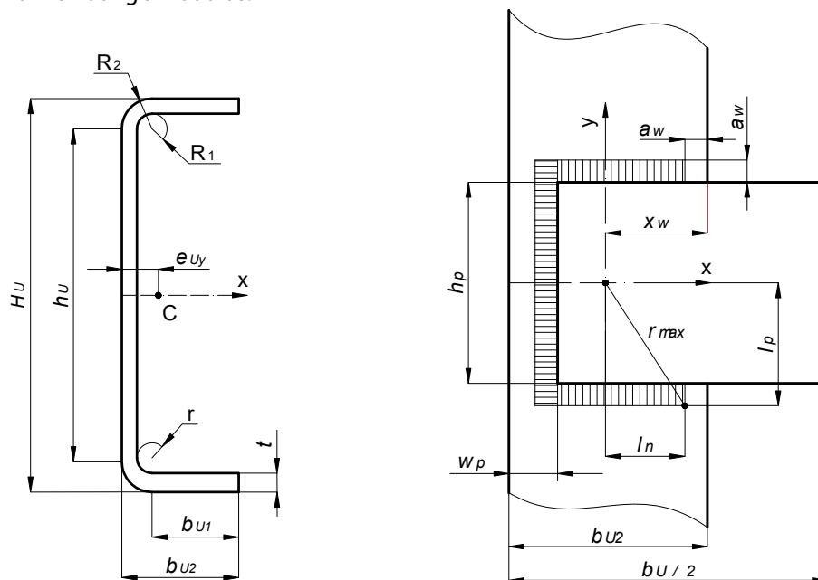
Figure 2: Cold-formed channel section
