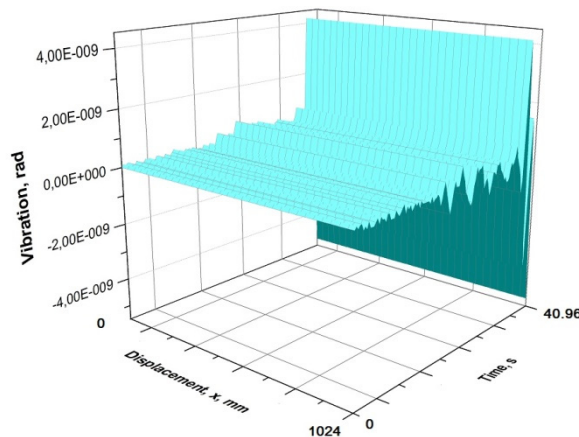
Figure 5. Torsional vibrations of the stabilizer's torsion bar
