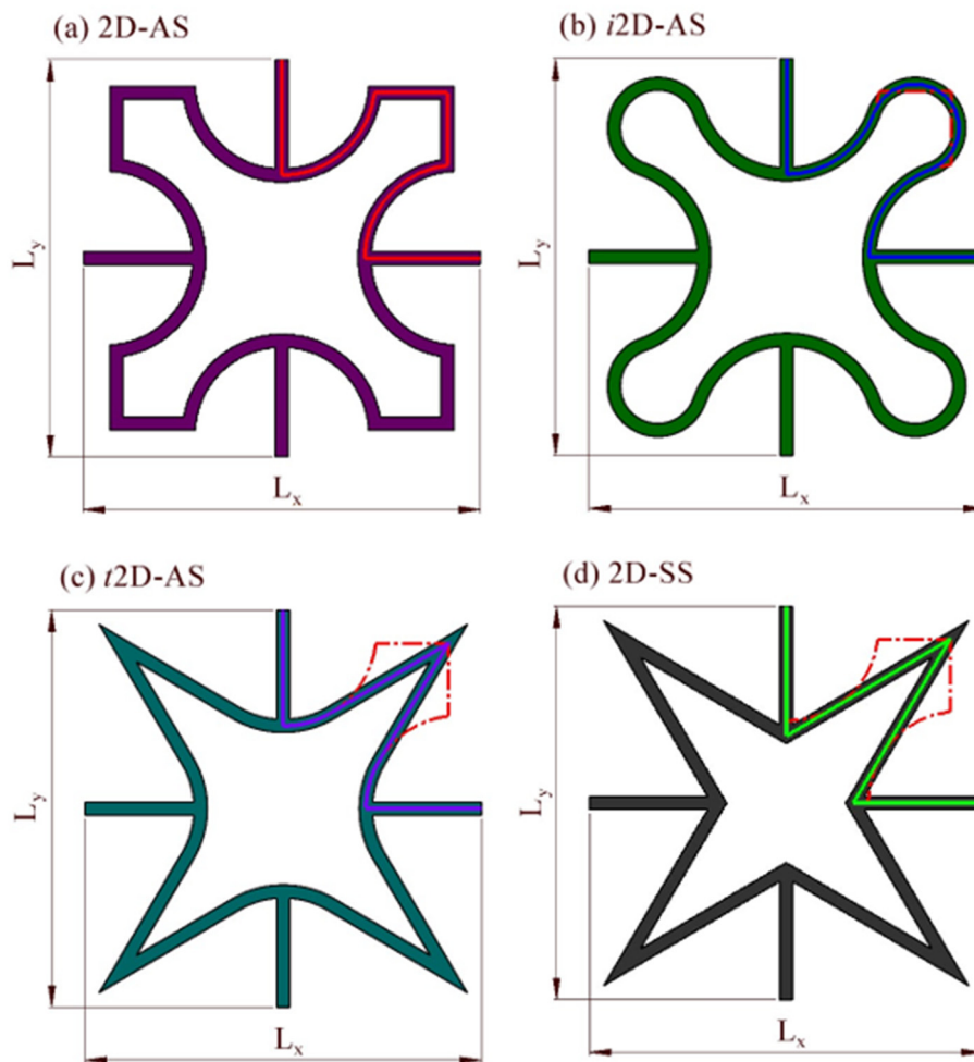
Figure 1: Geometrical parameters of Star-Shaped Structures [5,6,9]: (a) 2D-AS; (b) i 2D-AS; (c) t 2D-AS; (c) 2D-SS
