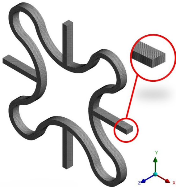
Figure 4: Generated mesh for the i2D-AS structure.
