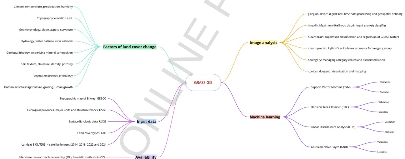
Figure 4: Schematic workflow of image processing and data analysis in GRASS GIS. Source: author.
