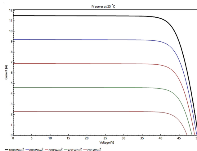
Figure 6: The current-voltage (IV) curve for JTSgh455 W module
