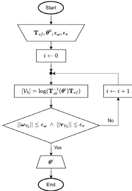
Algorithm 1. Newton-Raphson numerical method in the robots space frame
