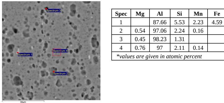
Figure 2. SEM-EDS analysis of the sample peak aged at 200°C for 4 hours
