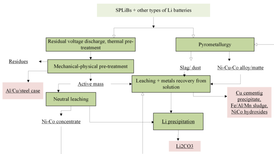
Figure 1. General scheme for industrial SPLiBs recycling
