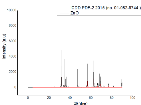
Figure 2 Diffractogram of ZnO nanoparticles
