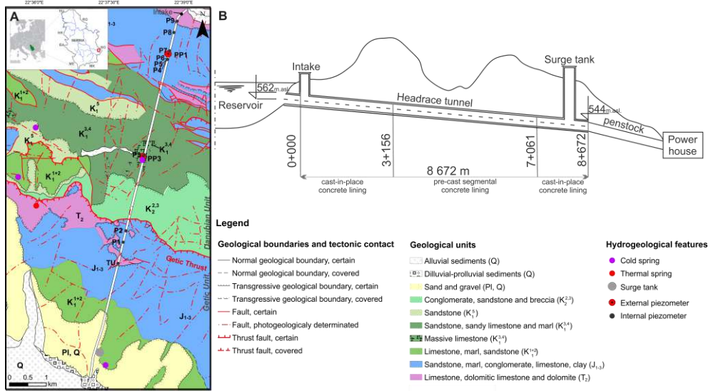
Fig. 1. (A) Geological sketch map of the study area (Andjelković et al., 1975); (B) Schematic representation of the Pirot HPP tunnel.
